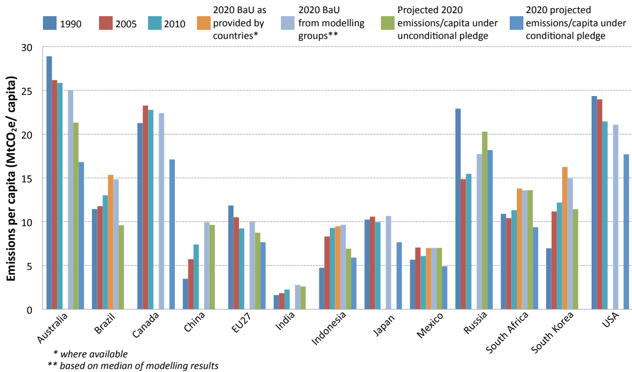
Figure 2.8. Year 1990, 2005, 2010 and 2020 greenhouse gas emissions per capita for G20 countries that have made pledges. Note that European Union countries are taken as a group. For emissions, see figure 2.6. Source: UN medium population numbers; UN (2011).
