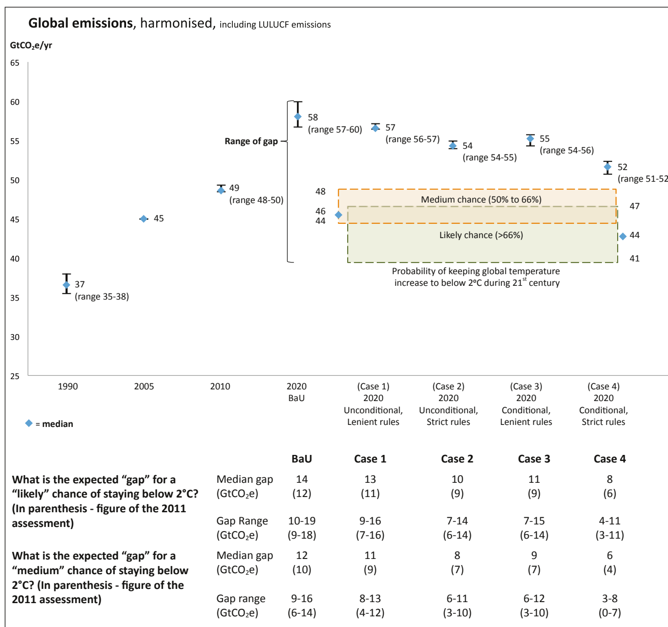
Figure 3.2 Summary of the gaps that result from four different interpretations of how the pledges are followed, and for a “likely” (greater than 66%) and a “medium” (50-66%) chance of staying below 2°C.
